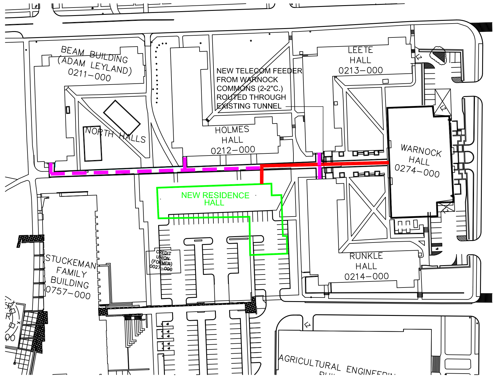
TELECOMMUNICATIONS SITE PLAN - NORTH HALLS SCALE: 1" = 100'
