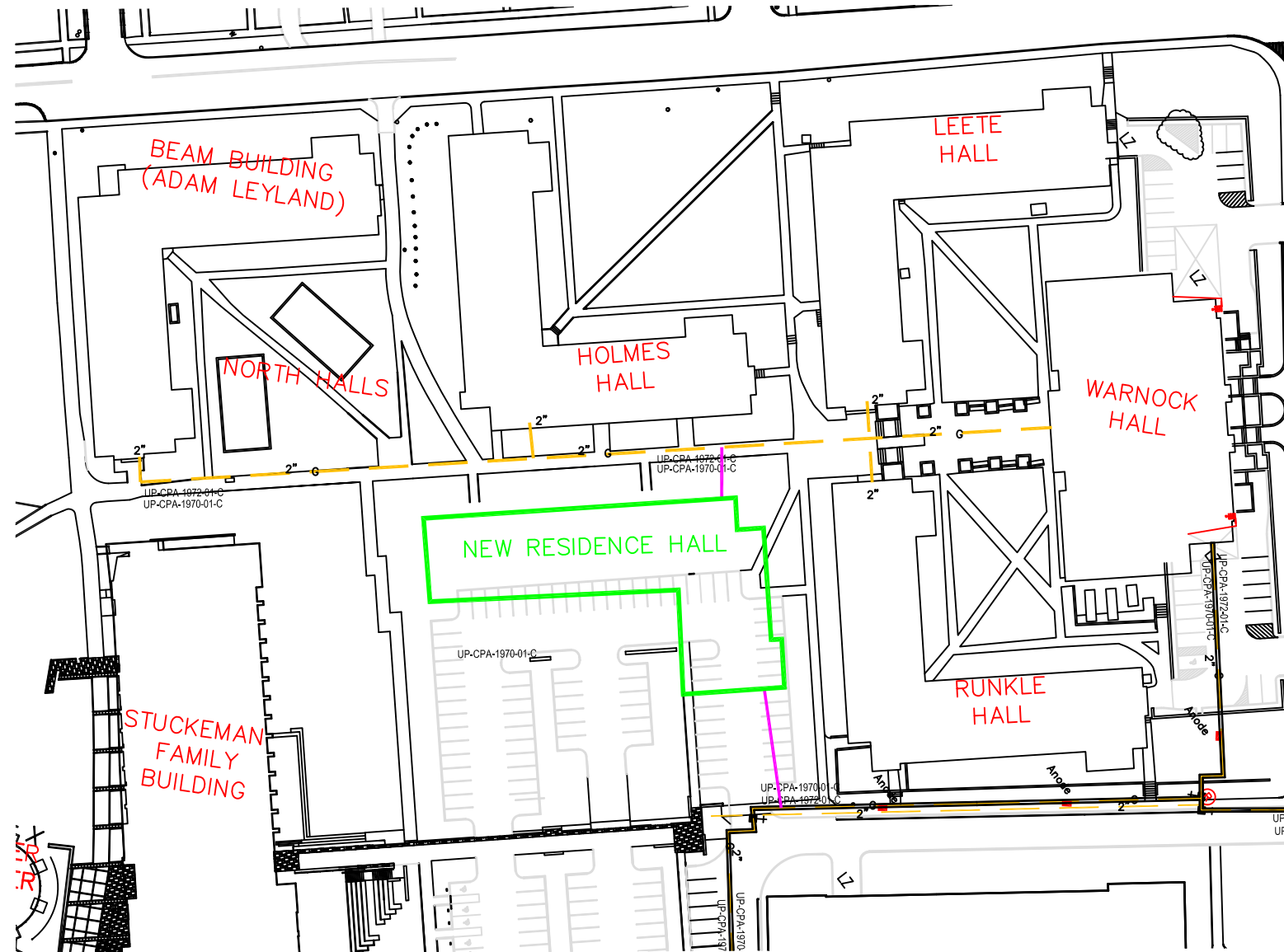
NATURAL GAS SYSTEM OVERLAY - NORTH HALLS
