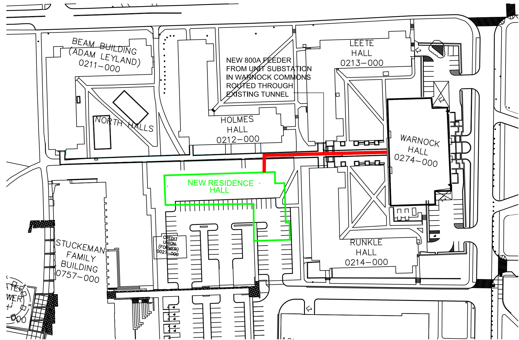
ELECTRICAL SITE PLAN - NORTH HALLS
