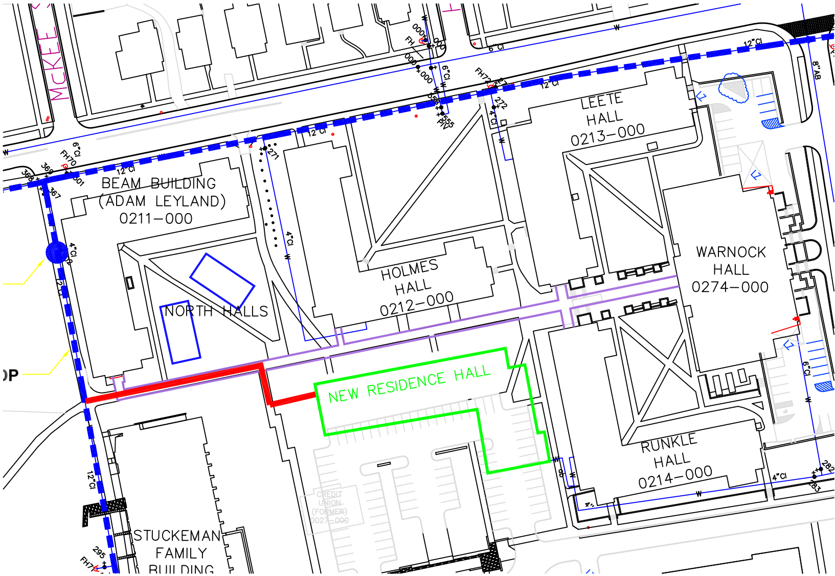
FIRE PROTECTION SITE PLAN - NORTH HALLS
