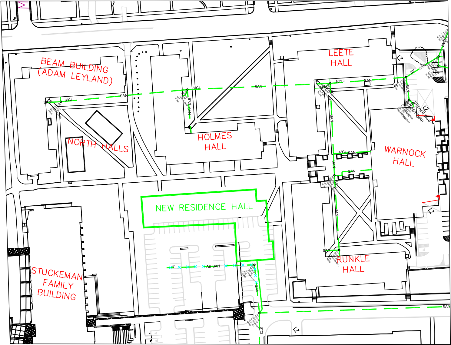
SANITARY SEWER OVERLAY - NORTH HALLS SCALE: 1" = 100'
